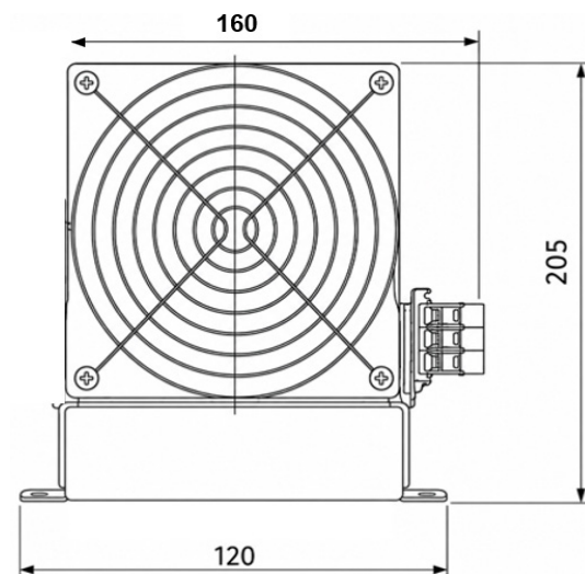
TECHNICAL DRAWING (SPECIFICATION IN MM)
