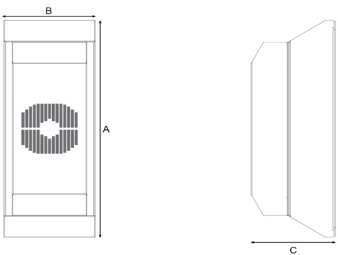
Wall mounted-Version 920105
