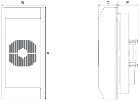
Recessed-Version 920005
